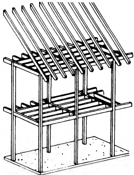
4 Timber frame
